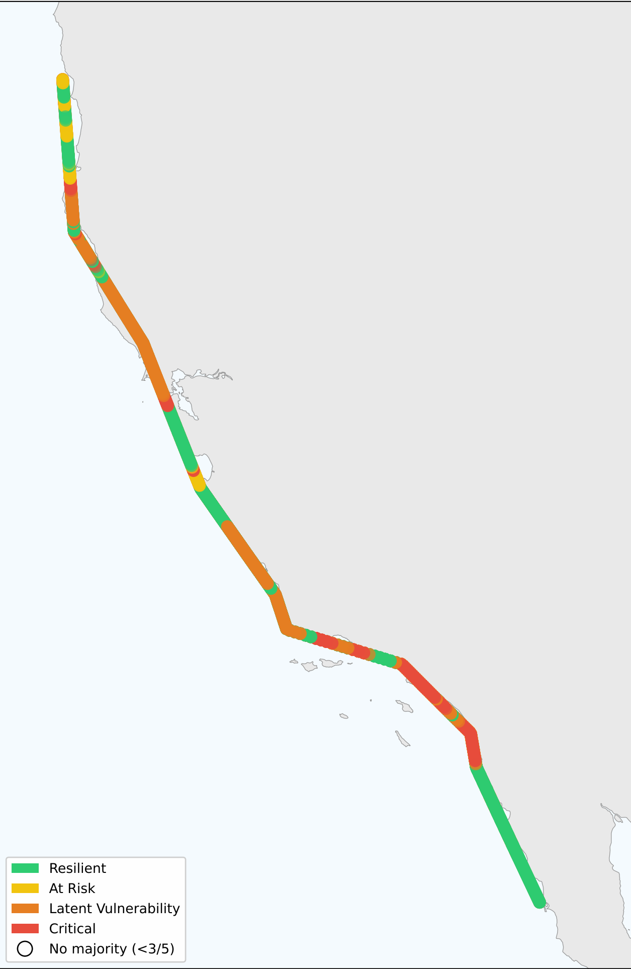
Per-GCM resilience classification — model-agreement map (color = modal class across 5 GCMs; opacity = agreement)
