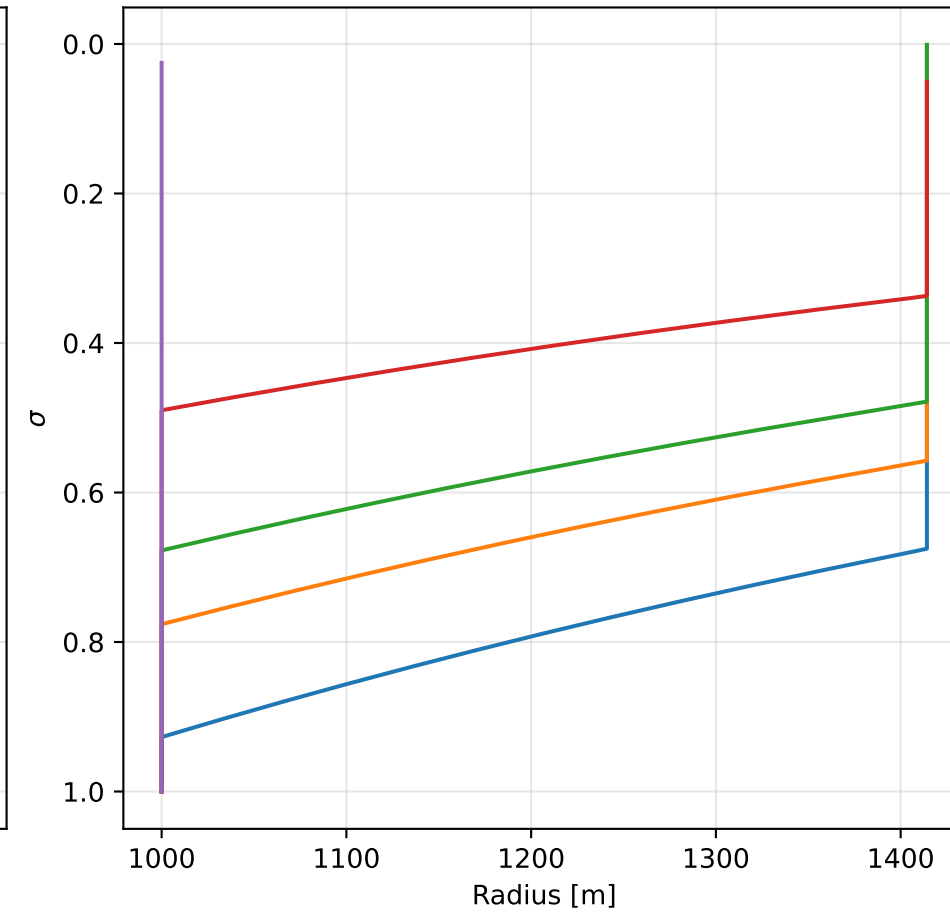
Plume Radius
