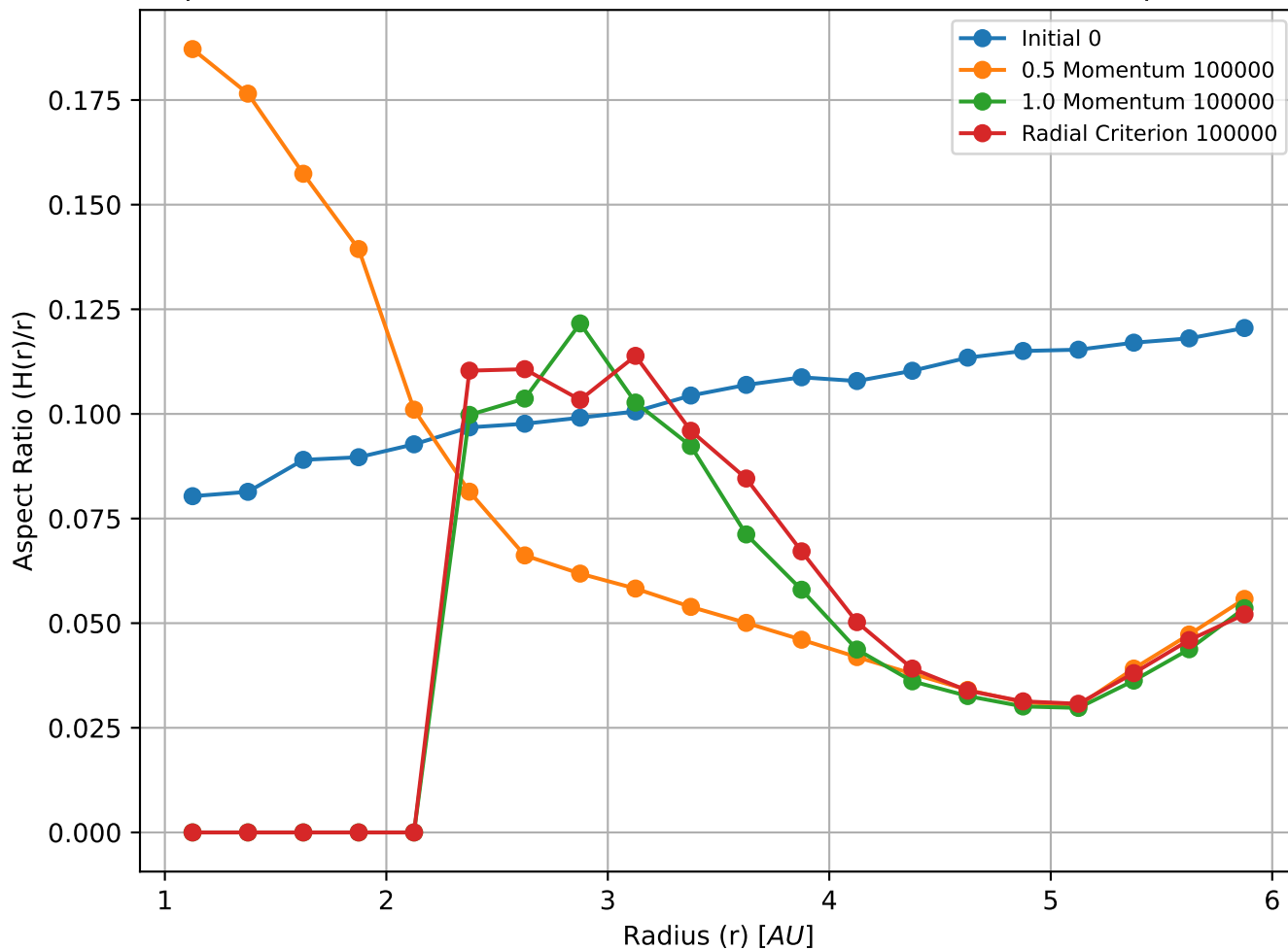
Aspect Ratio vs Radius of Different Accretion Criteria at Timestep 100000
