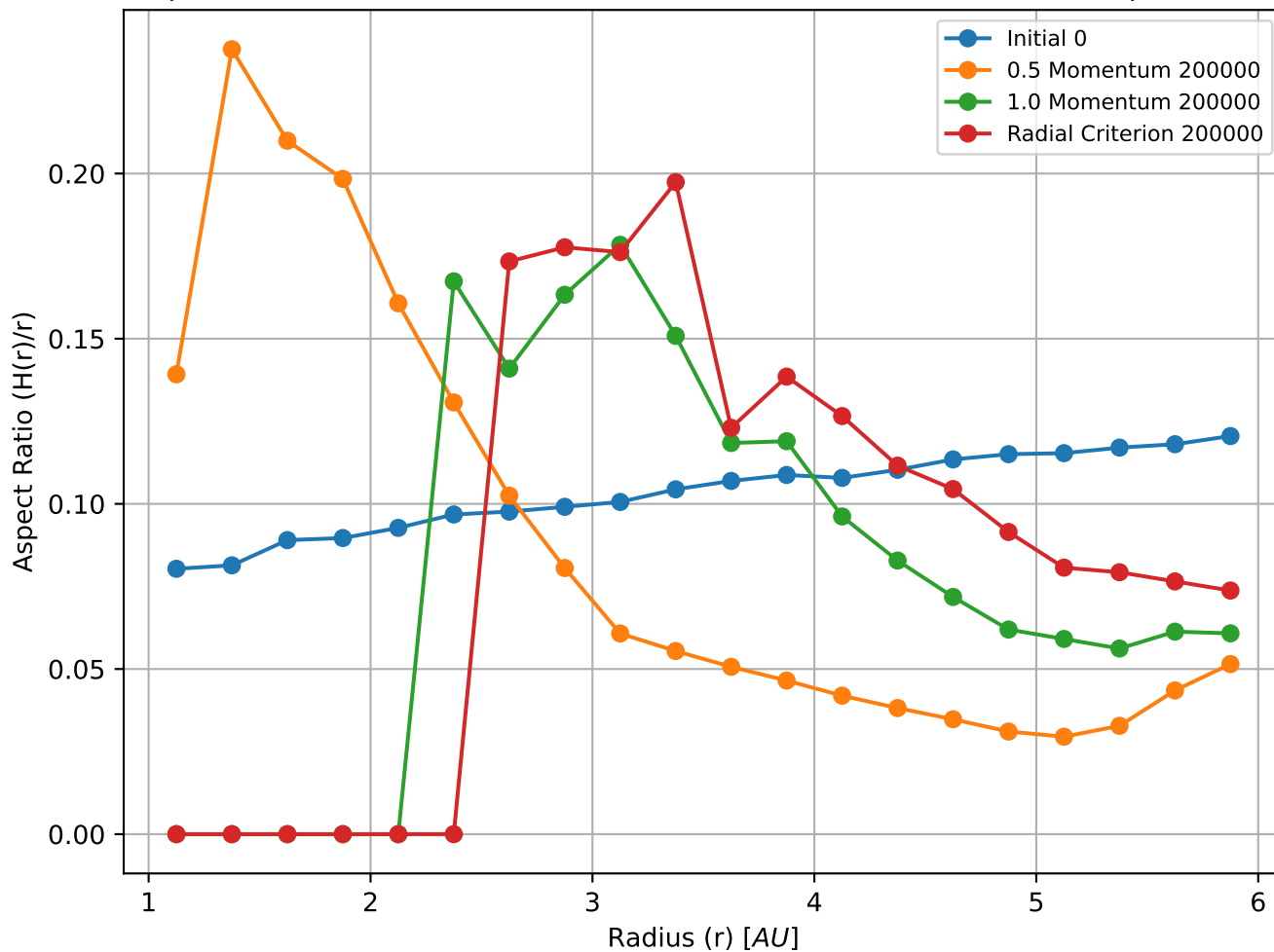
Aspect Ratio vs Radius of Different Accretion Criteria at Timestep 200000
