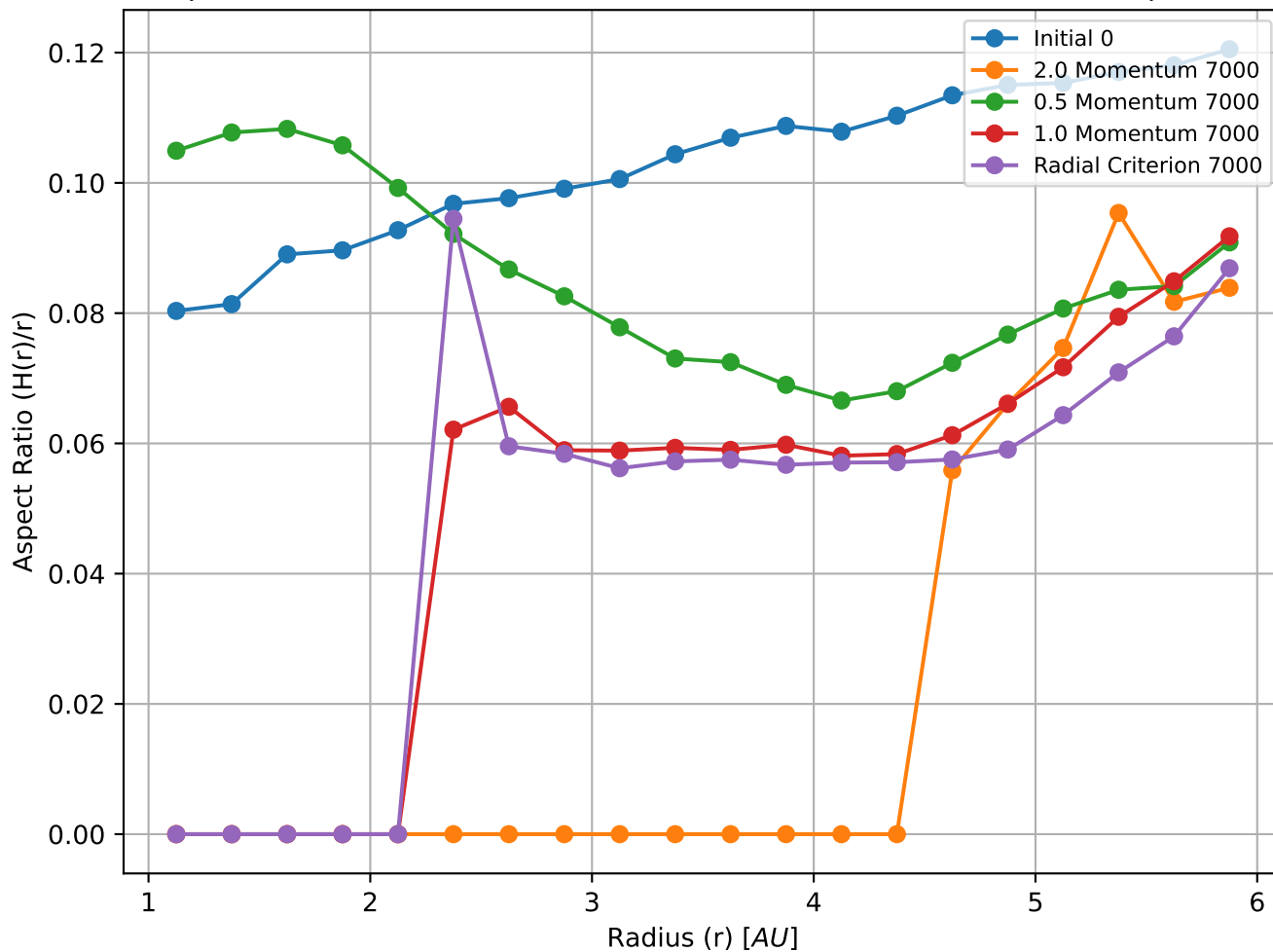
Aspect Ratio vs Radius of Different Accretion Criteria at Timestep 7000
