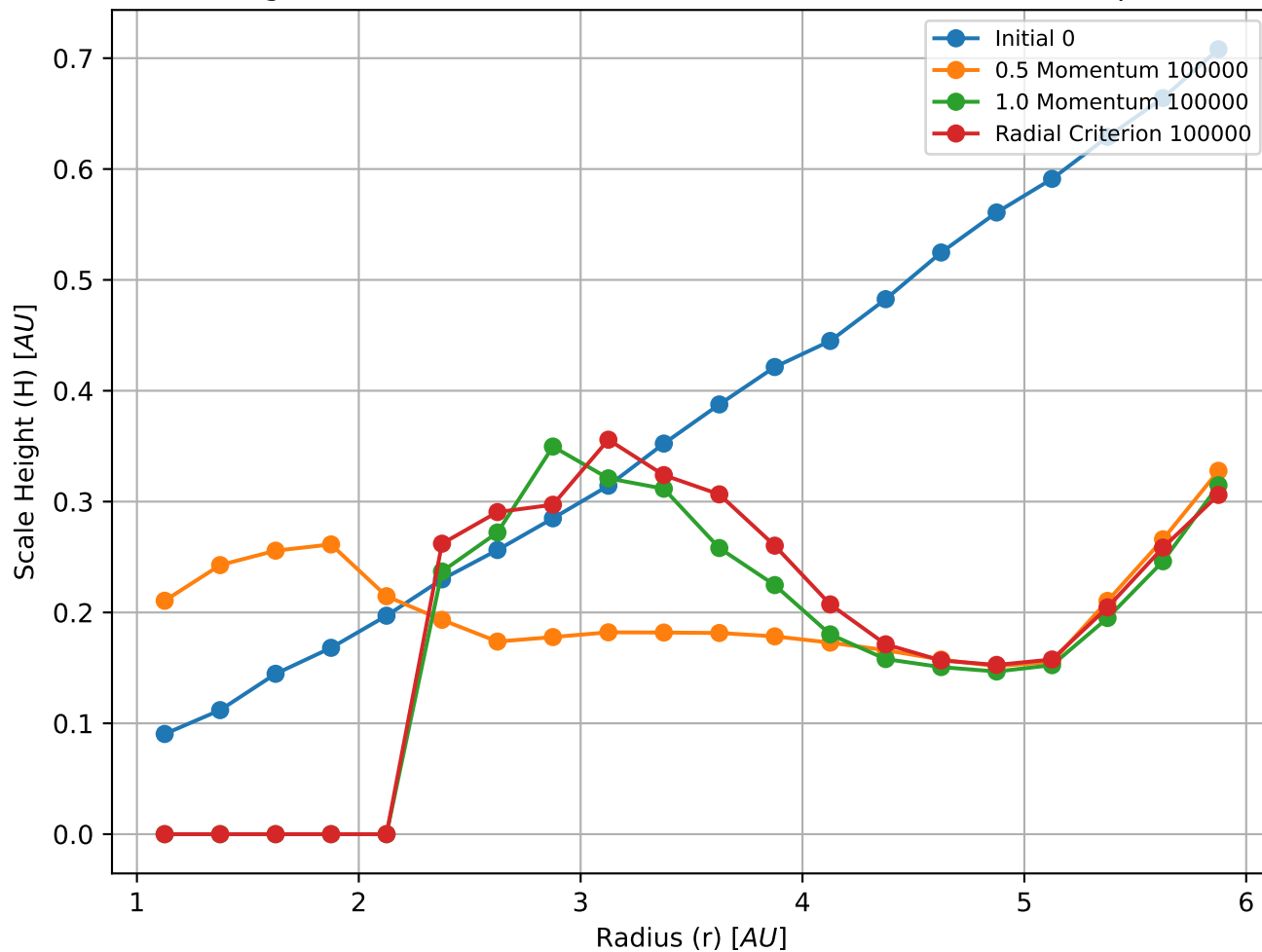
Scale Height vs Radius of Different Accretion Criteria at Timestep 100000
