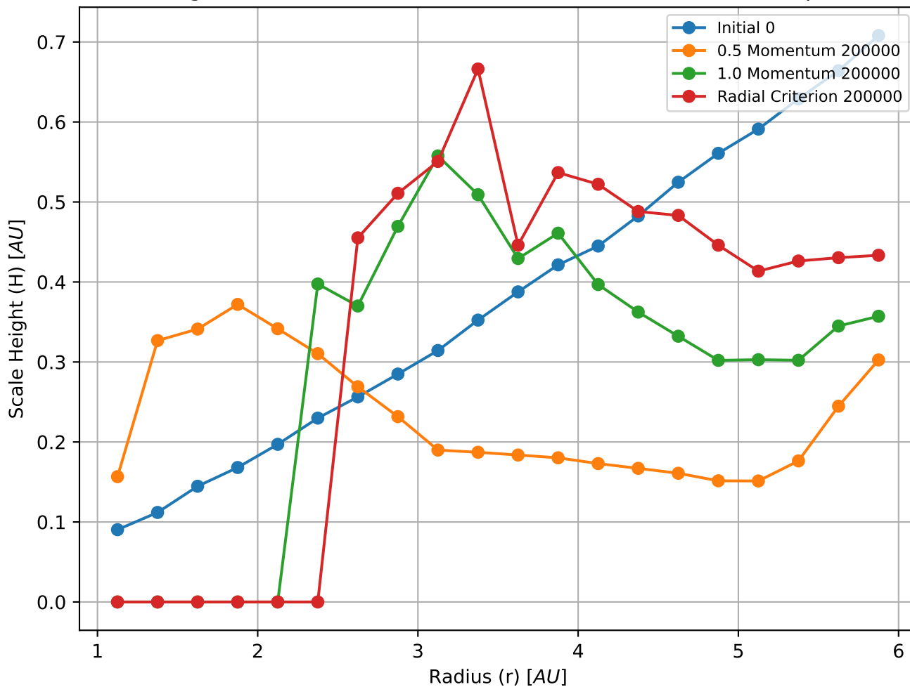
Scale Height vs Radius of Different Accretion Criteria at Timestep 200000
