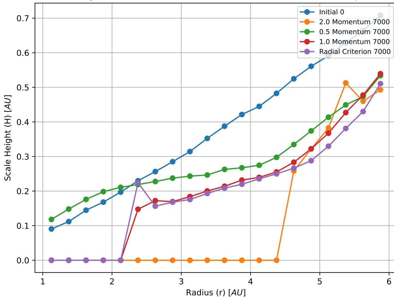
Scale Height vs Radius of Different Accretion Criteria at Timestep 7000
