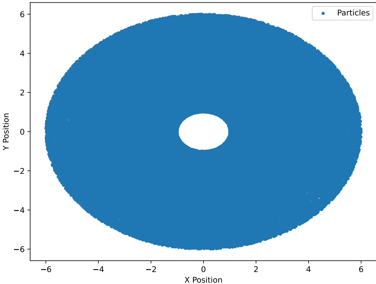
Particles at Timestep 0, No Accretion ( \beta=2\pi )
