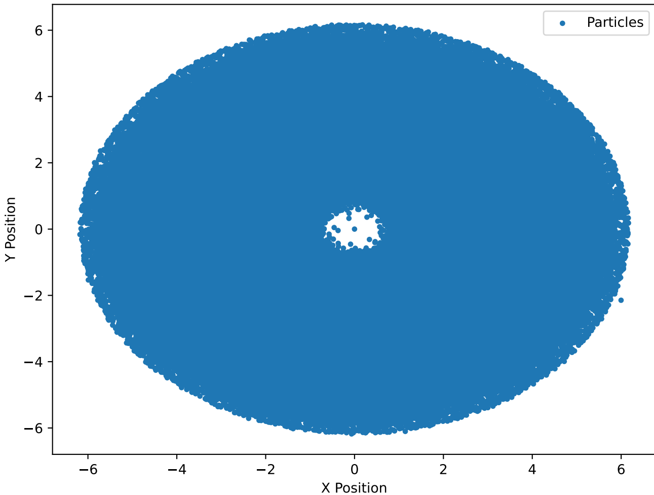
Particles at Timestep 10000, No Accretion ( \beta=2\pi )
