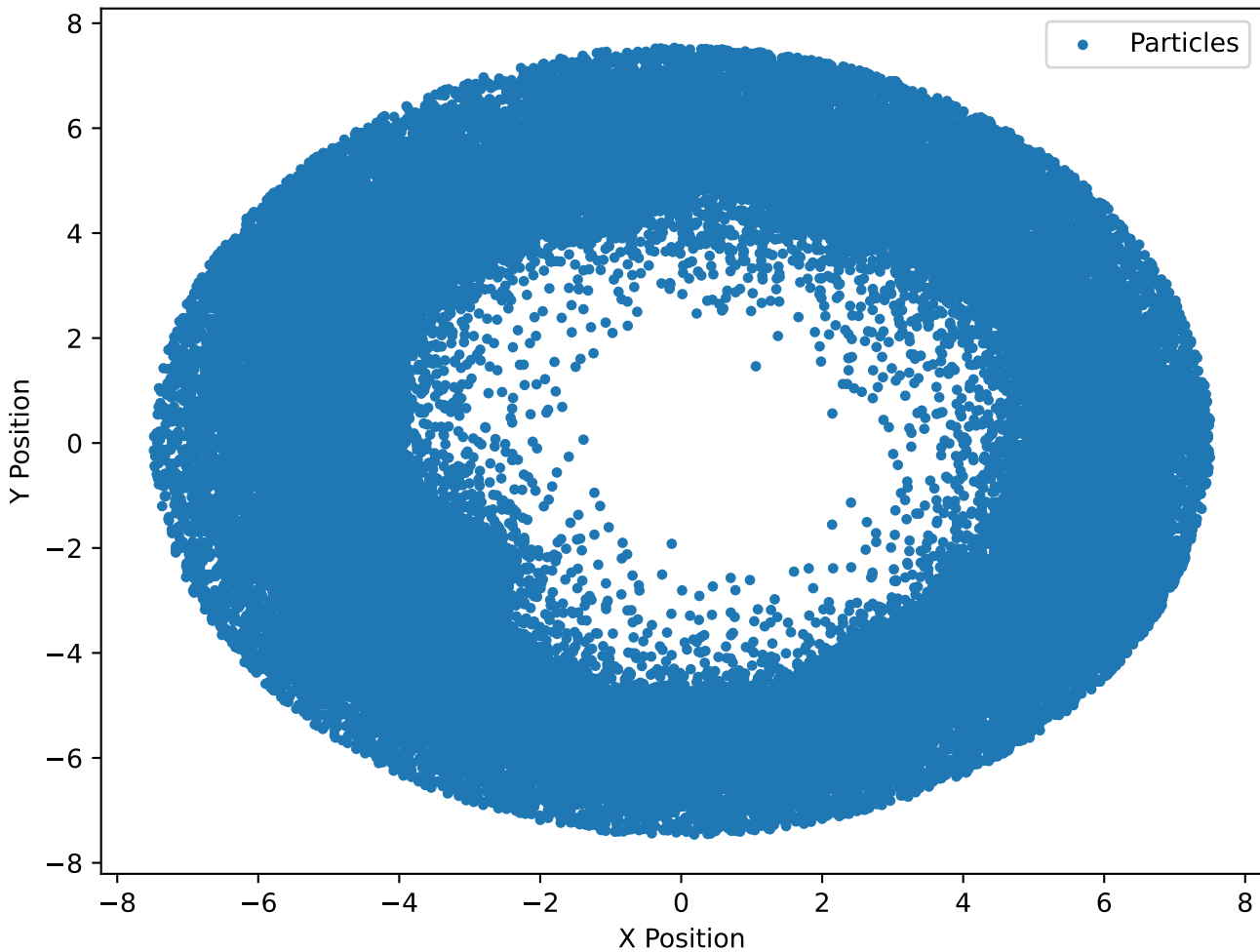
Particles at Timestep 250000, No Accretion ( \beta=2\pi )
