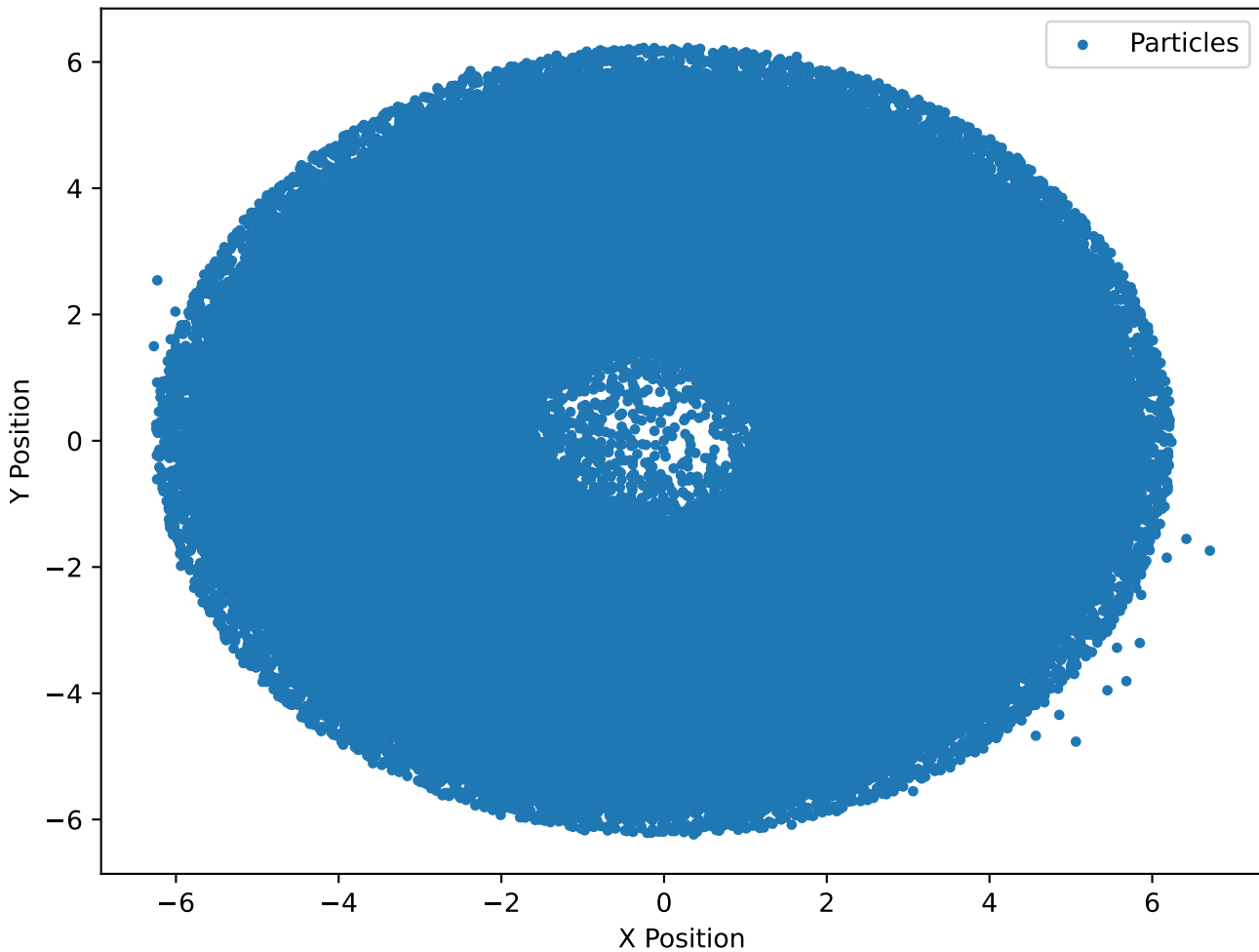
Particles at Timestep 40000, No Accretion ( \beta=2\pi )
