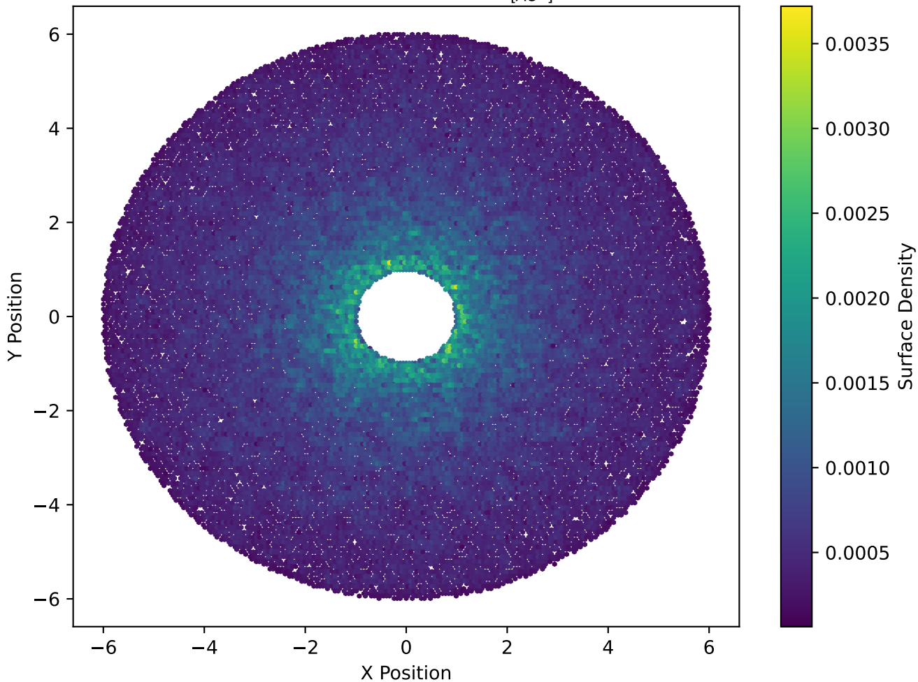
Surface Density at Timestep 0 \frac{[M_\odot]}{[AU^2]} , ( \beta=2\pi )
