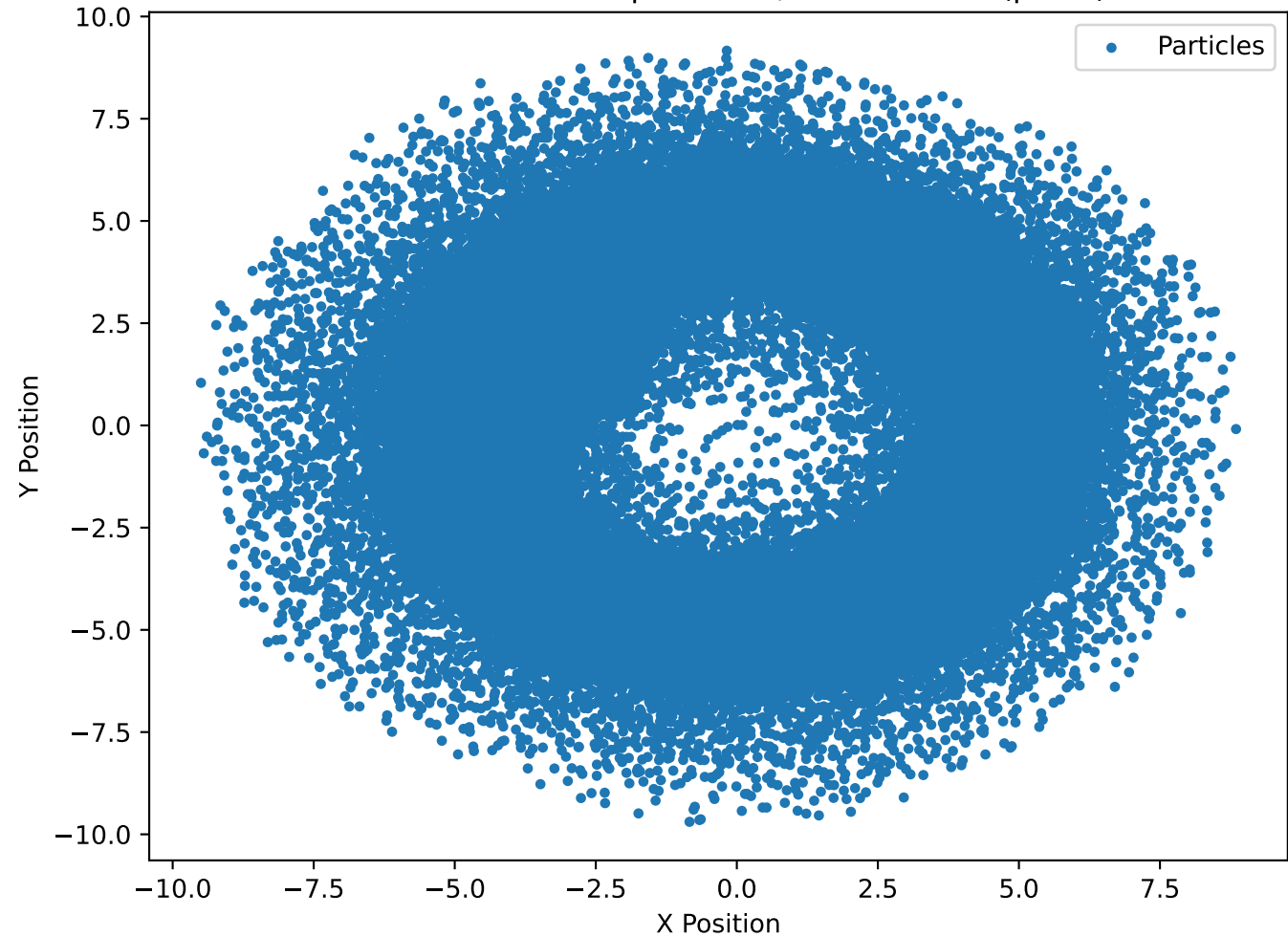
Particles at Timestep 150000, No Accretion ( \beta=2\pi )
