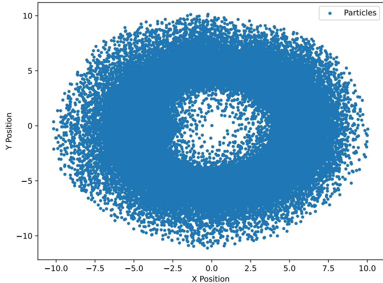
Particles at Timestep 200000, No Accretion ( \beta=2\pi )
