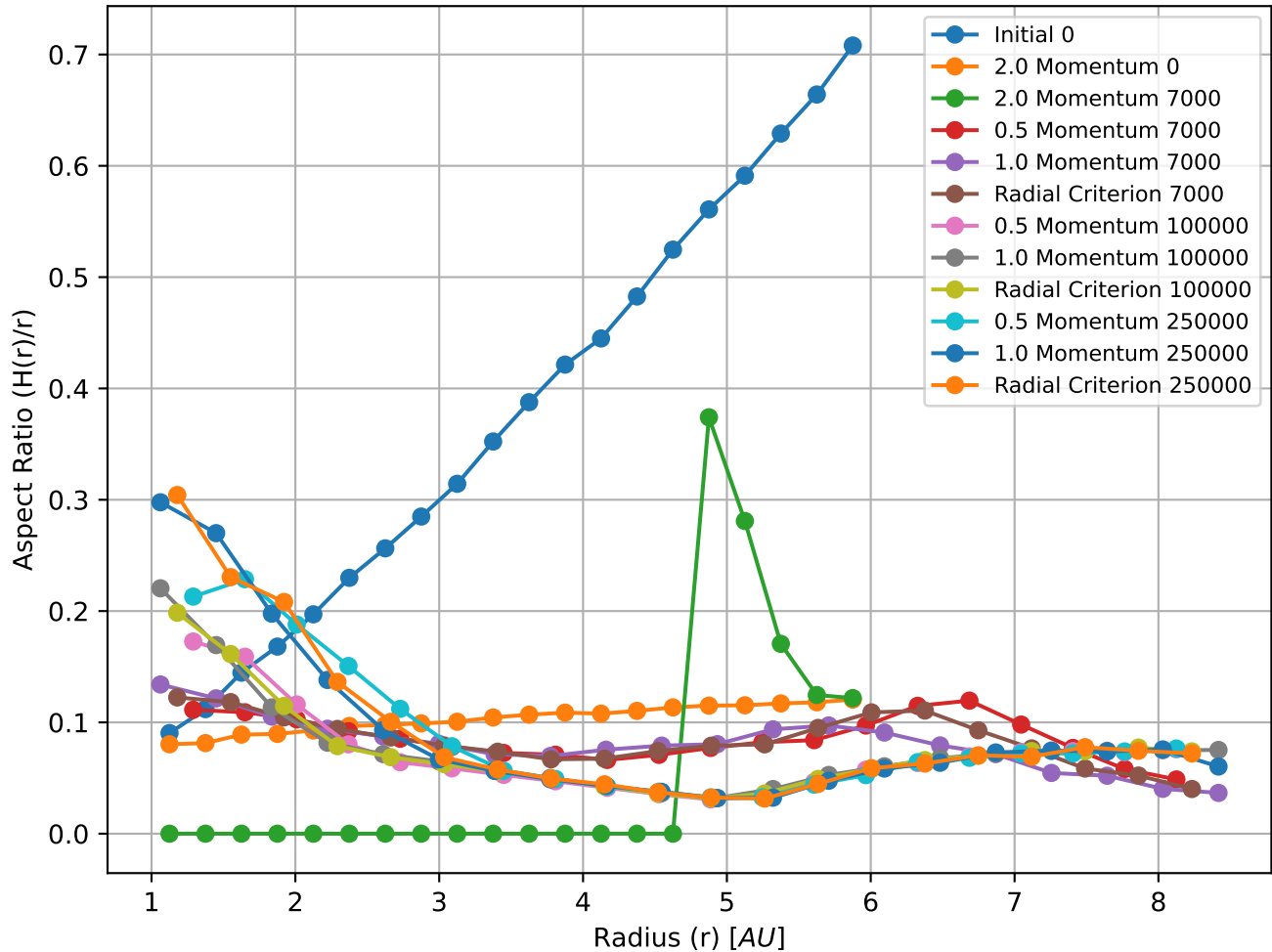
Aspect Ratio vs Radius of Different Accretion Criteria
