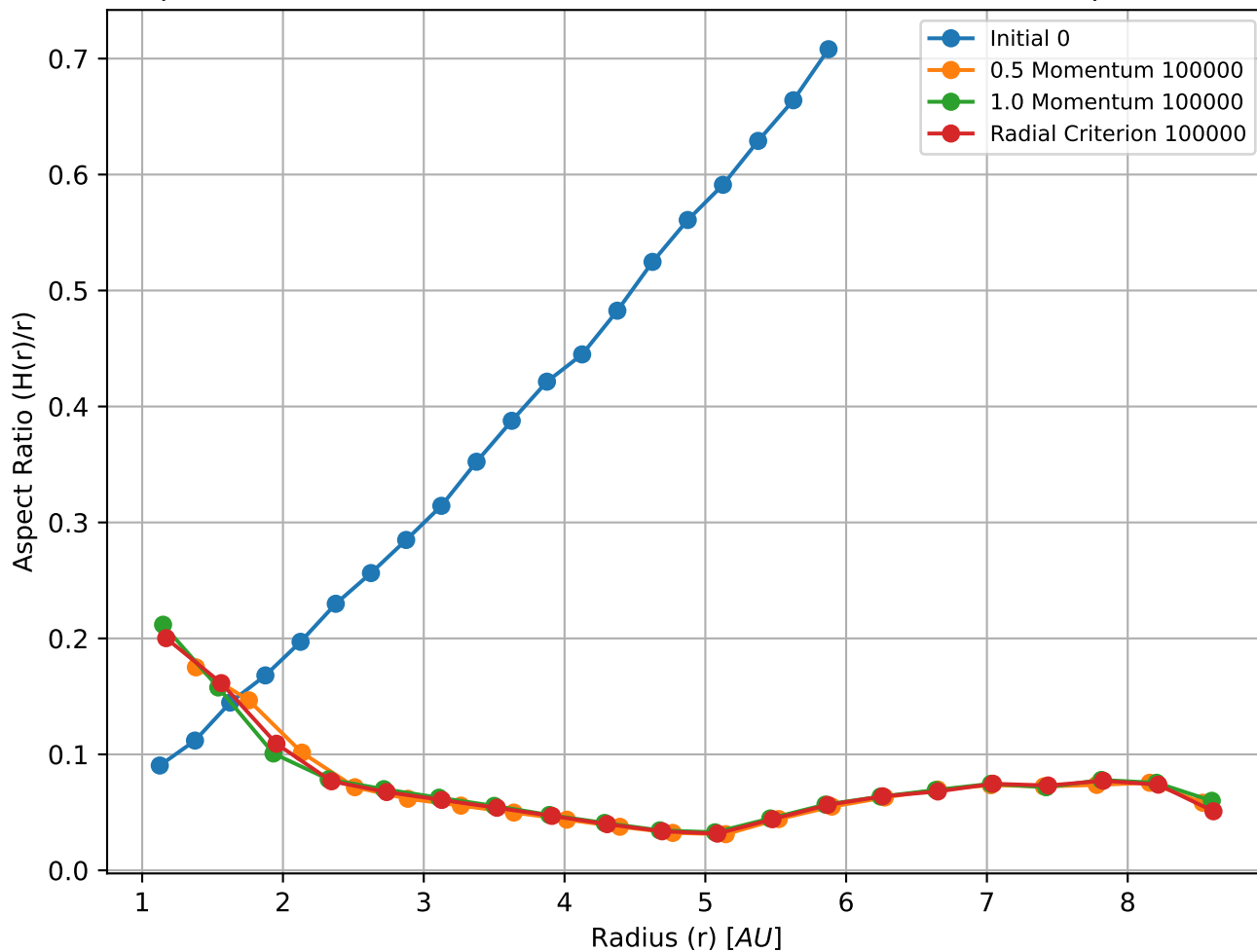
Aspect Ratio vs Radius of Different Accretion Criteria (Timestep 100000)
