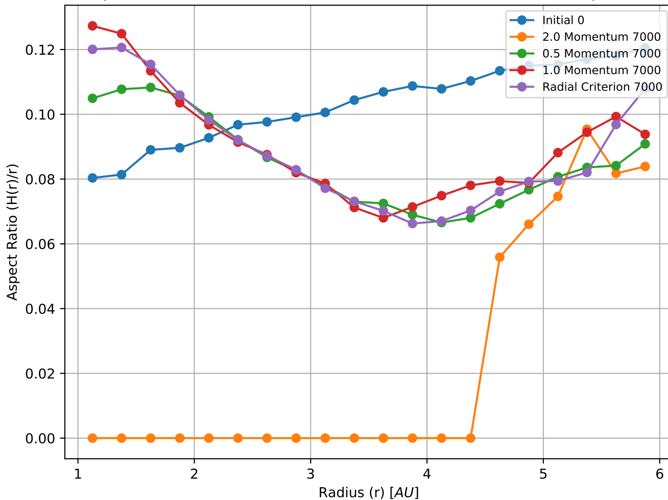
Aspect Ratio vs Radius of Different Accretion Criteria (Timestep 7000)
