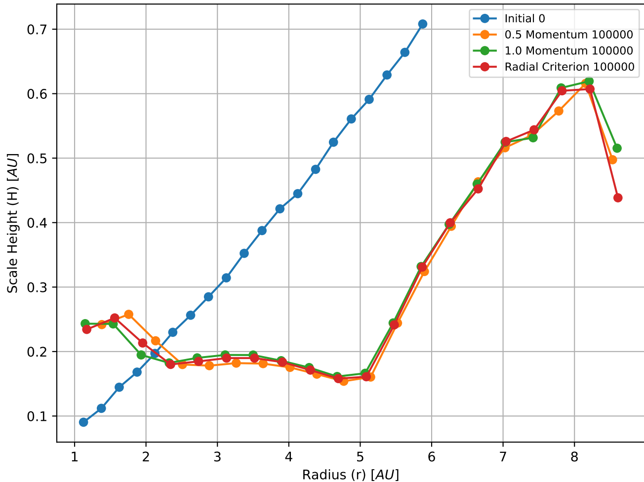
Scale Height vs Radius of Different Accretion Criteria
