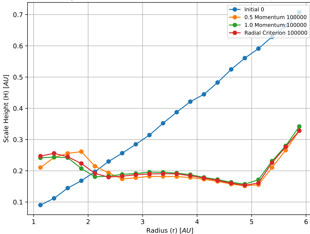
Scale Height vs Radius of Different Accretion Criteria Timestep 100000
