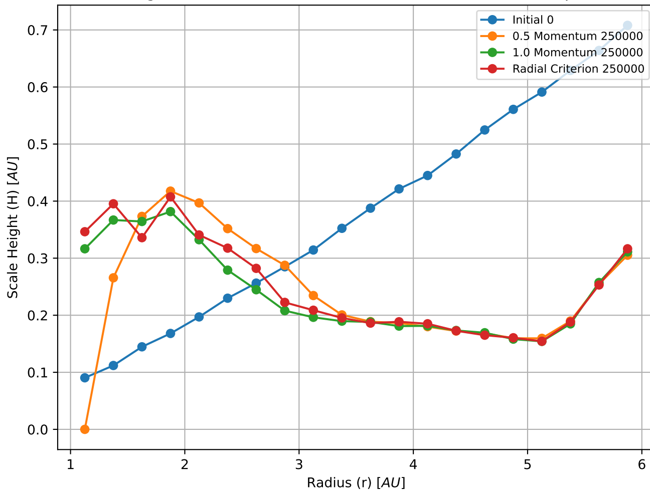
Scale Height vs Radius of Different Accretion Criteria Timestep 250000
