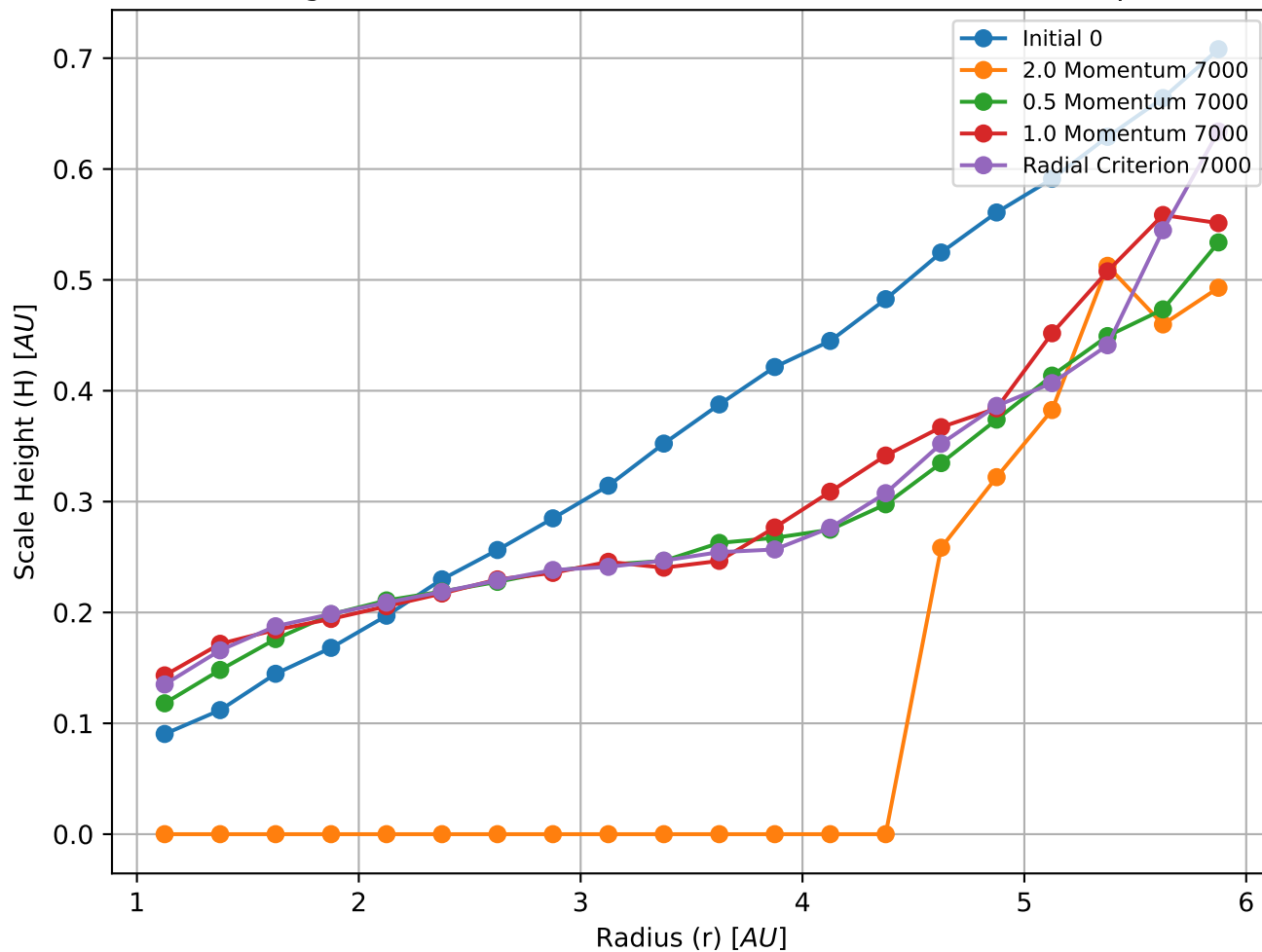
Scale Height vs Radius of Different Accretion Criteria Timestep 7000
