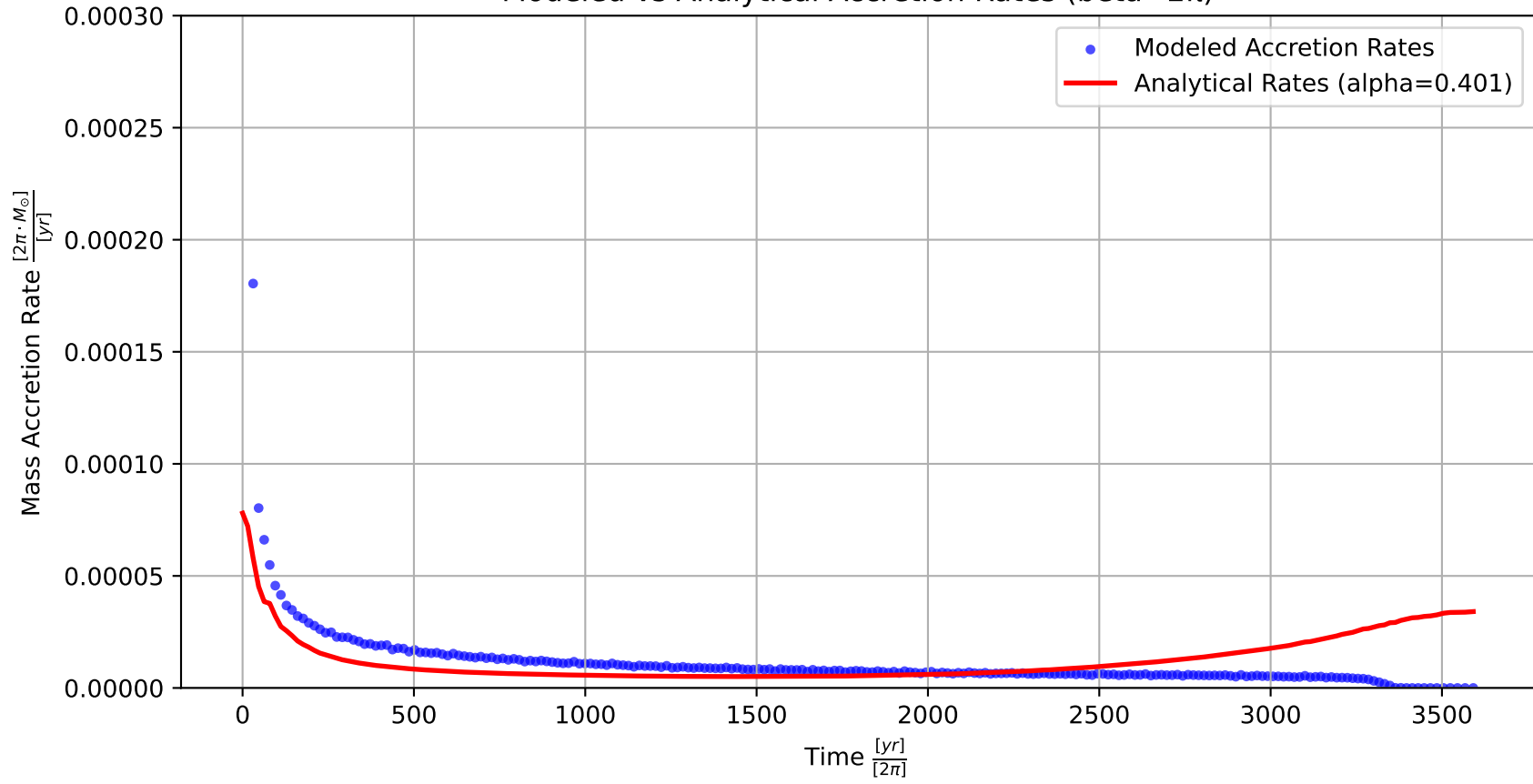
Modeled vs Analytical Accretion Rates (beta=2 \pi )
