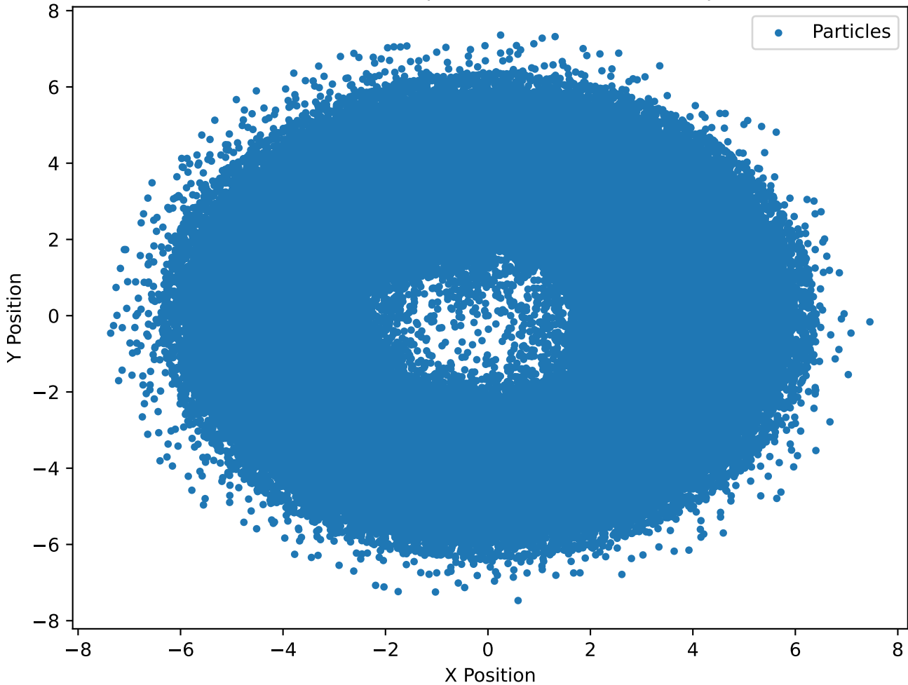
Particles at Timestep 100000, No Accretion ( \beta=2\pi )
