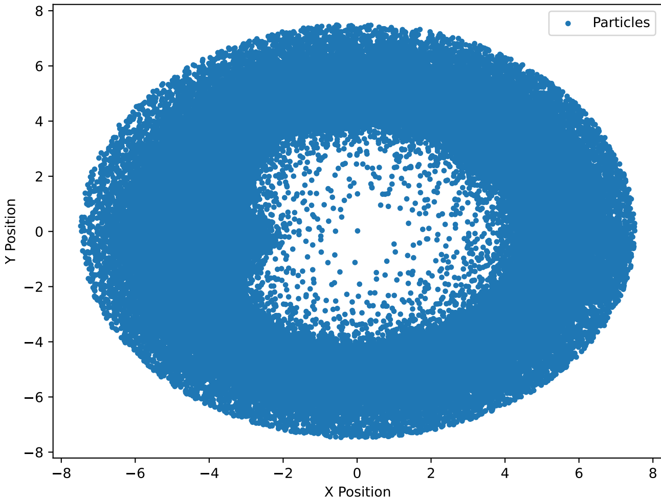
Particles at Timestep 200000, No Accretion ( \beta=2\pi )
