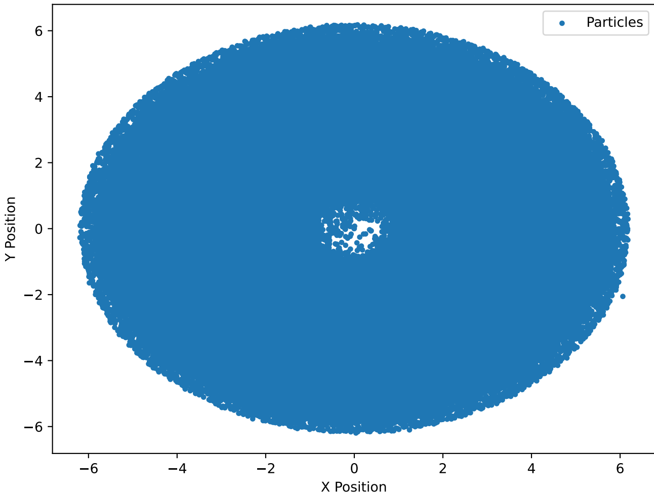
Particles at Timestep 20000, No Accretion ( \beta=2\pi )
