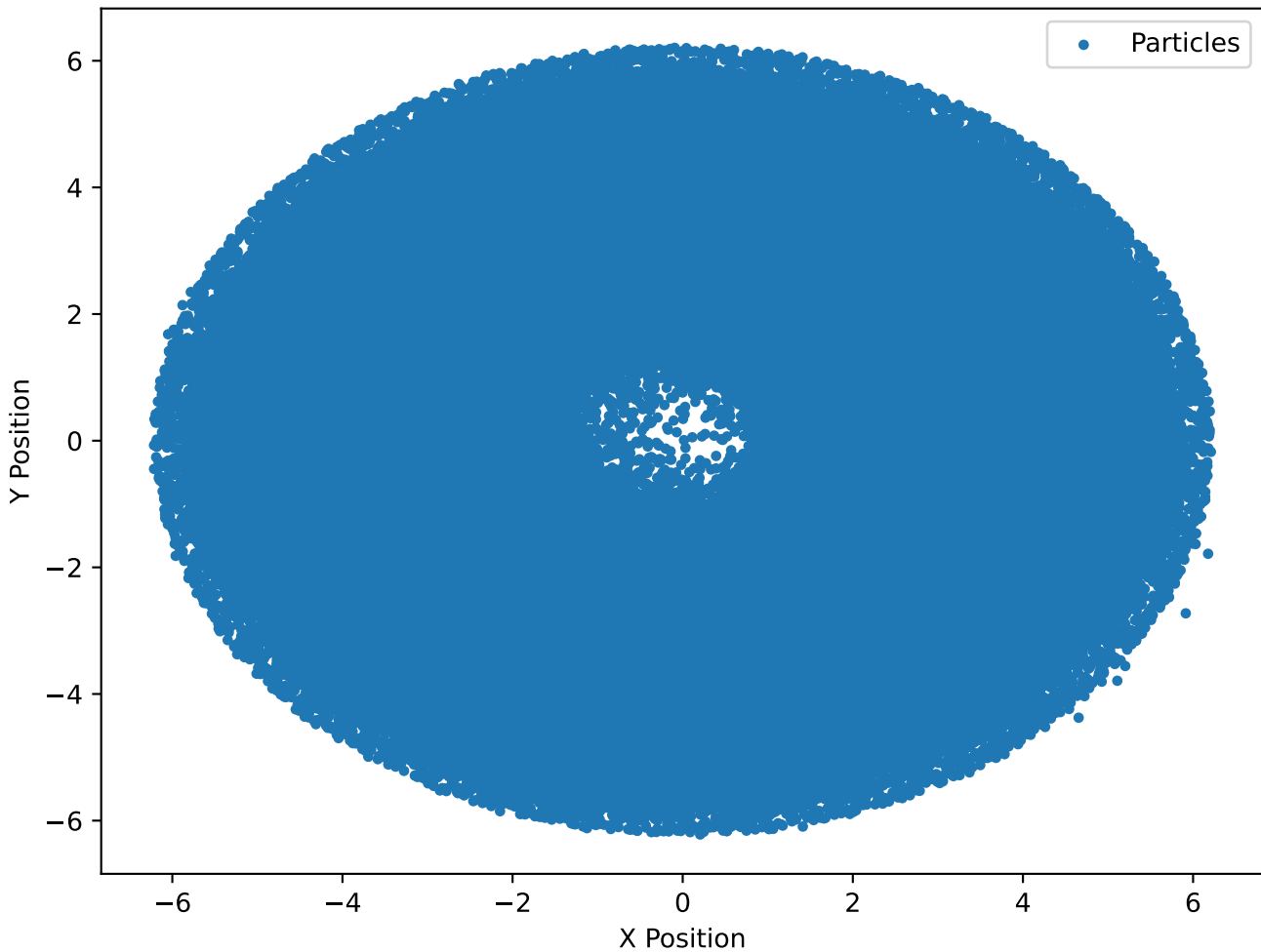
Particles at Timestep 25000, No Accretion ( \beta=2\pi )
