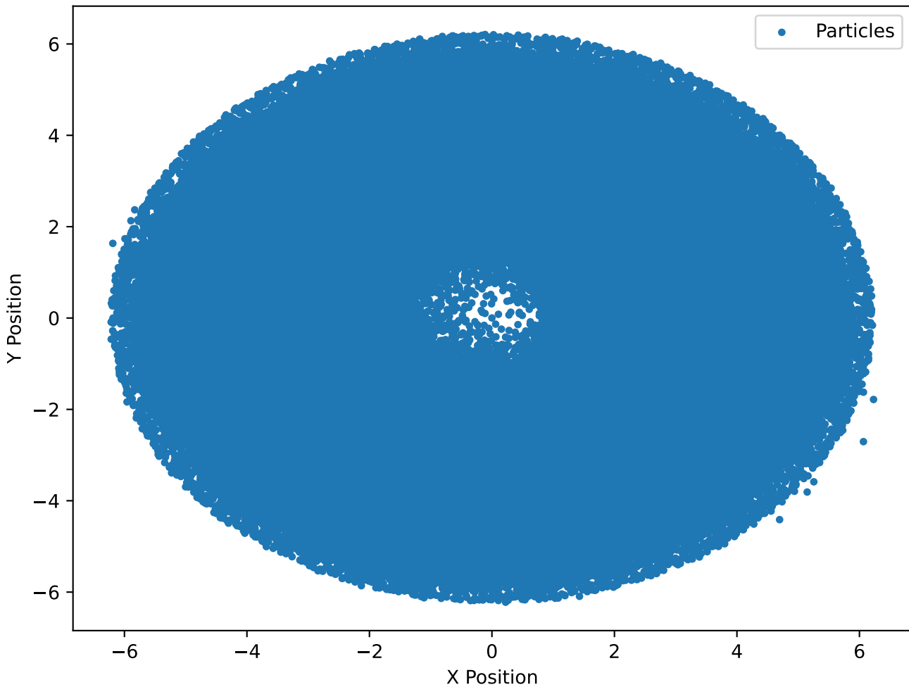
Particles at Timestep 30000, No Accretion ( \beta=2\pi )
