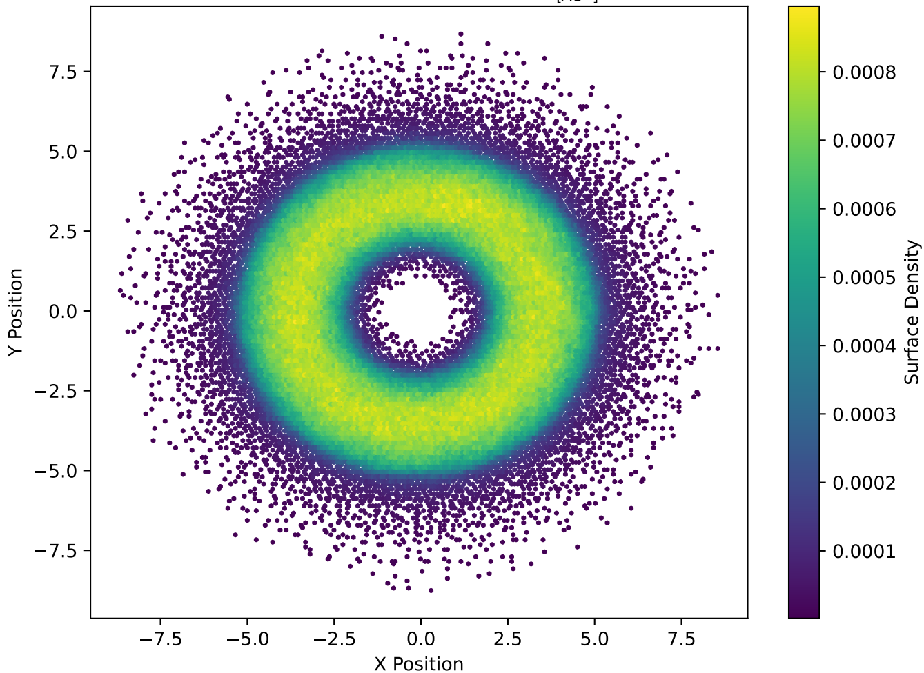
Surface Density at Timestep 100000 \frac{[M_\odot]}{[AU^2]} , ( \beta=2\pi )
