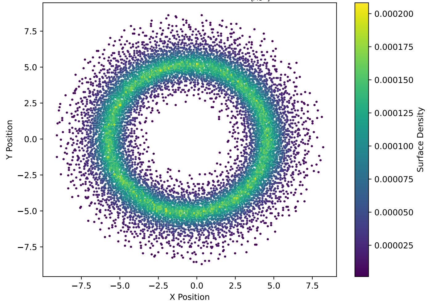
Surface Density at Timestep 200000 \frac{[M_\odot]}{[AU^2]} , ( \beta=2\pi )
