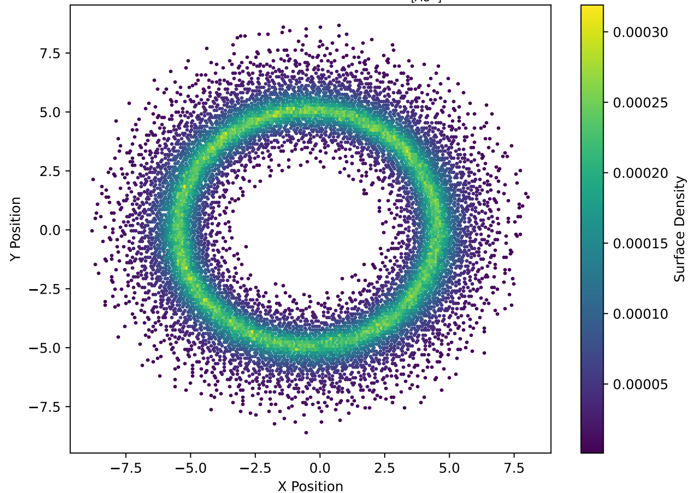
Surface Density at Timestep 150000 \frac{[M_{\odot}]}{[AU^2]} , ( \beta=2\pi )
