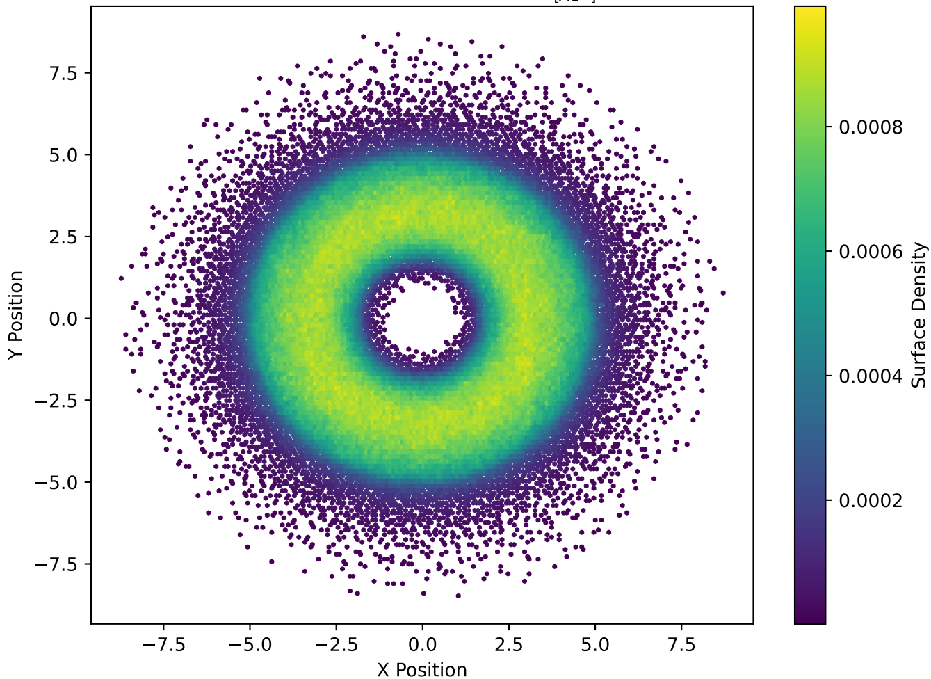
Surface Density at Timestep 50000 \frac{[M_{\odot}]}{[AU^2]} , ( \beta=2\pi )
