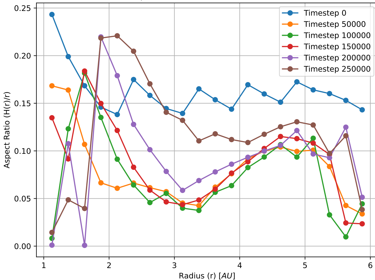
Aspect Ratio vs Radius, \beta = 2\pi
