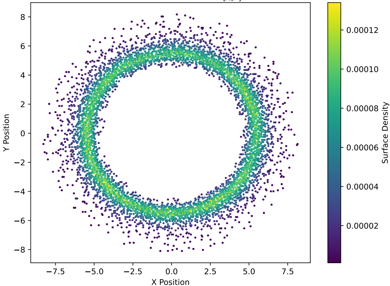
Surface Density at Timestep 2000 \frac{[M_{\odot}]}{[AU^2]} , ( \beta=2\pi )
