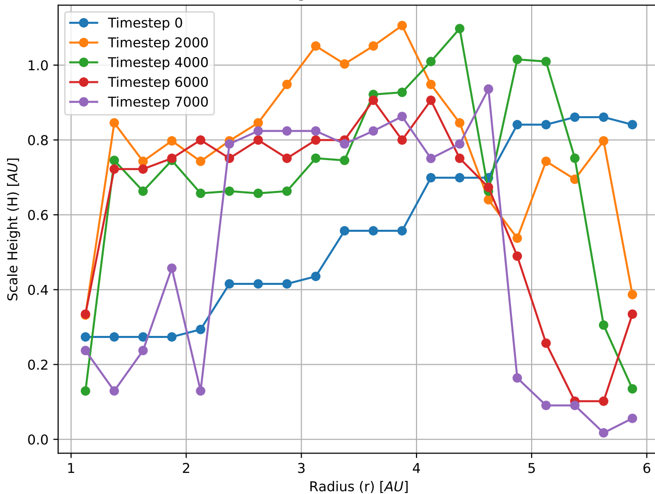
Scale Height vs Radius, \beta = 2\pi
