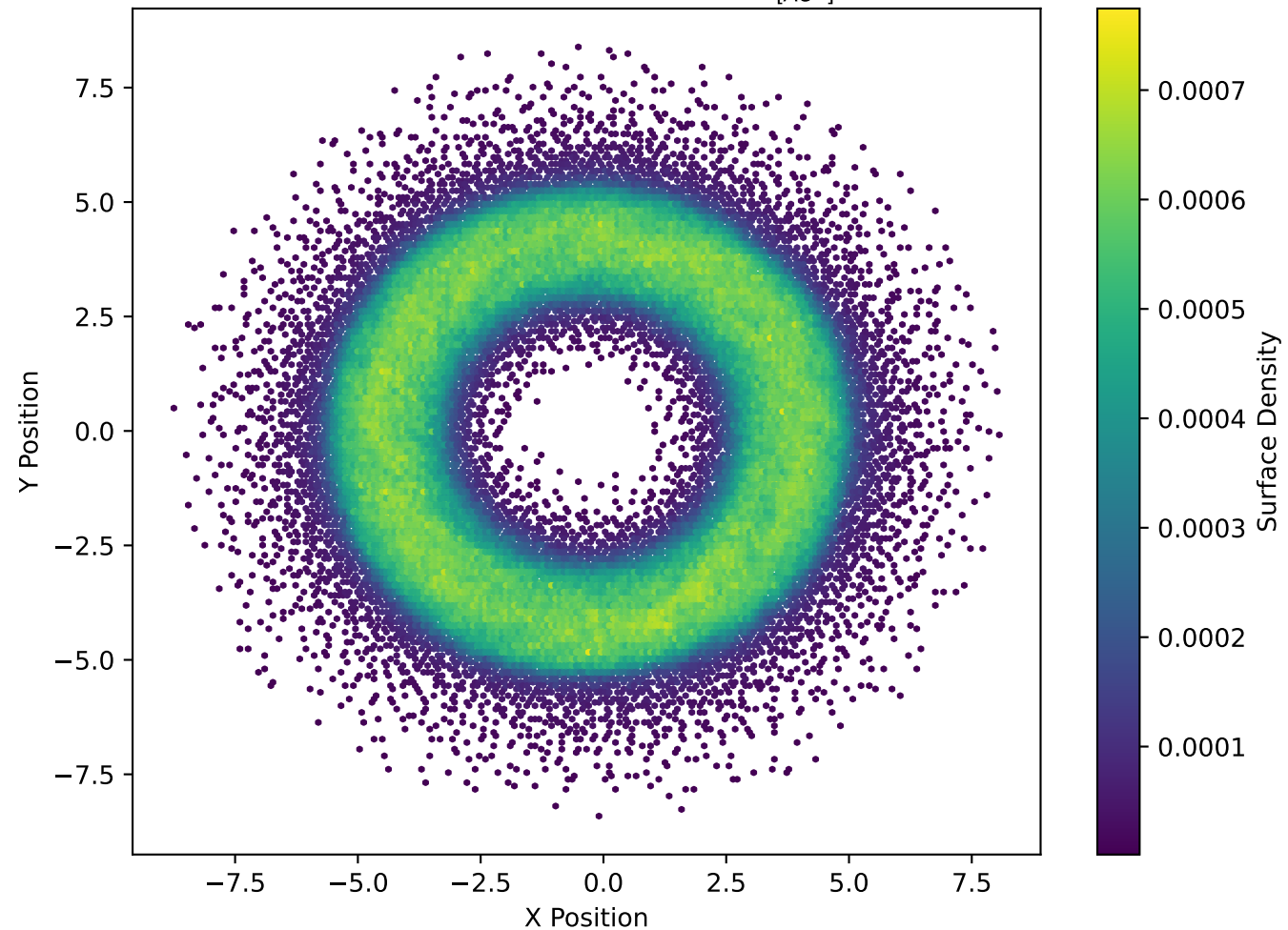
Surface Density at Timestep 200000 \frac{[M_\odot]}{[AU^2]} , ( \beta=2\pi )
