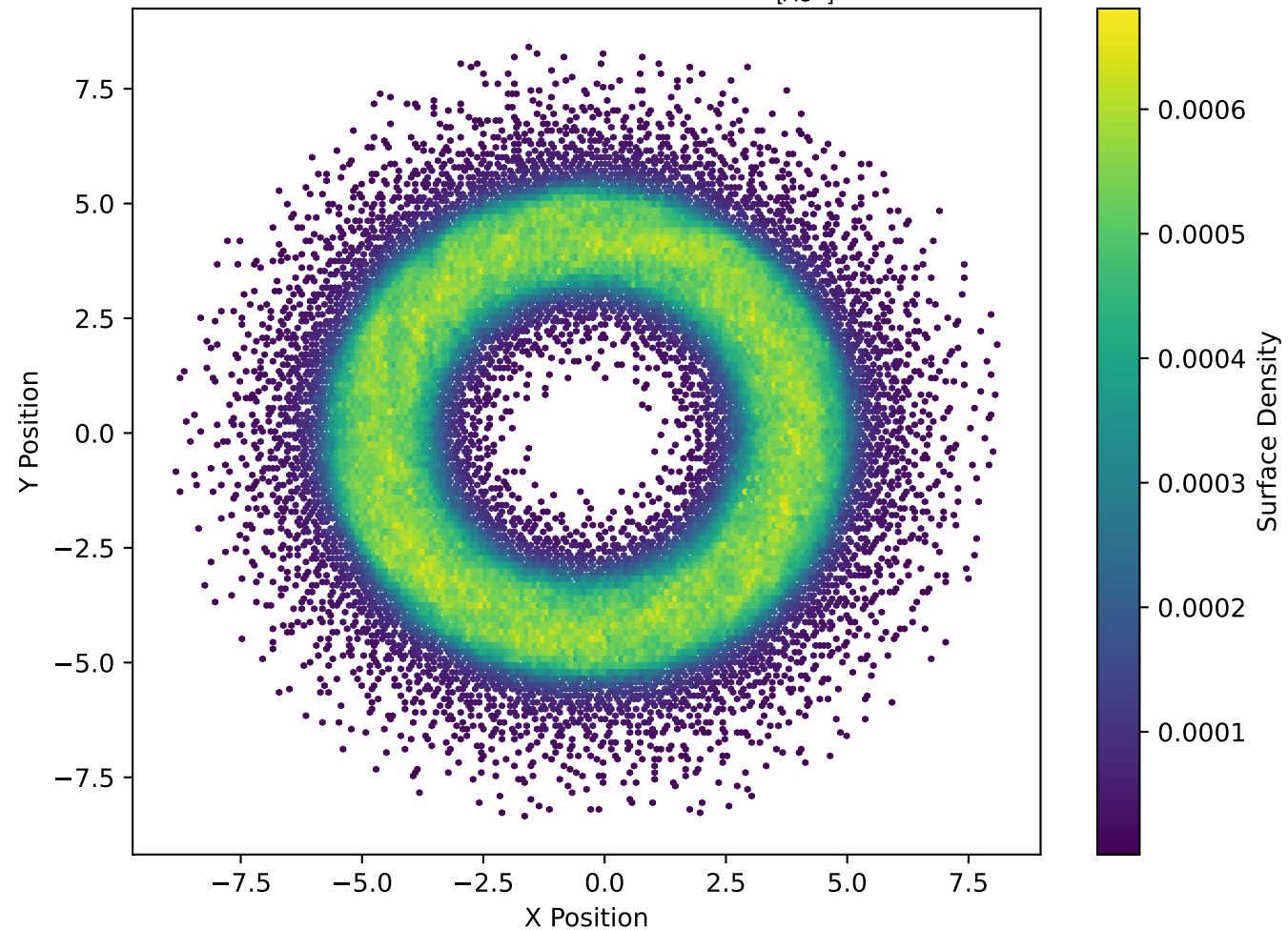
Surface Density at Timestep 250000 \frac{[M_\odot]}{[AU^2]} , ( \beta=2\pi )
