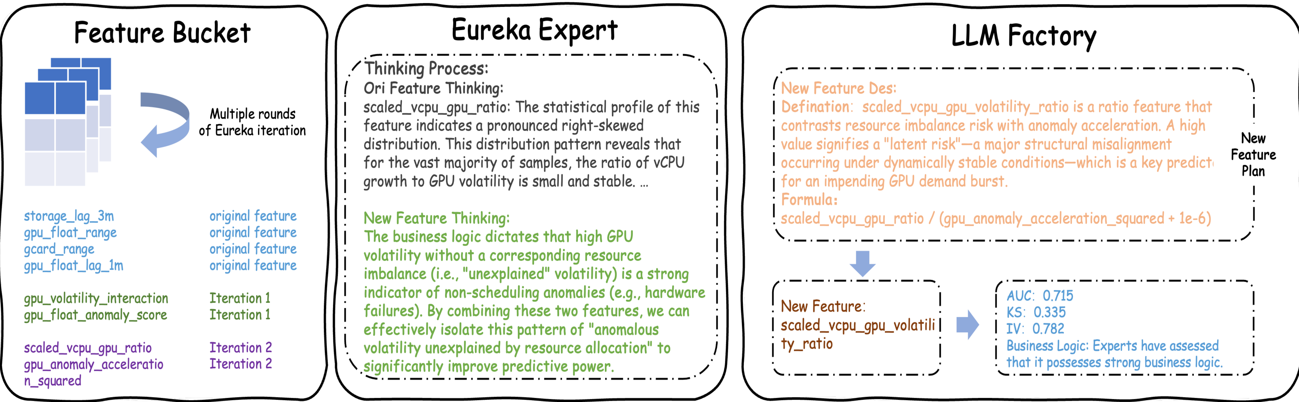
The process of obtaining high-quality features in EGS scenarios
