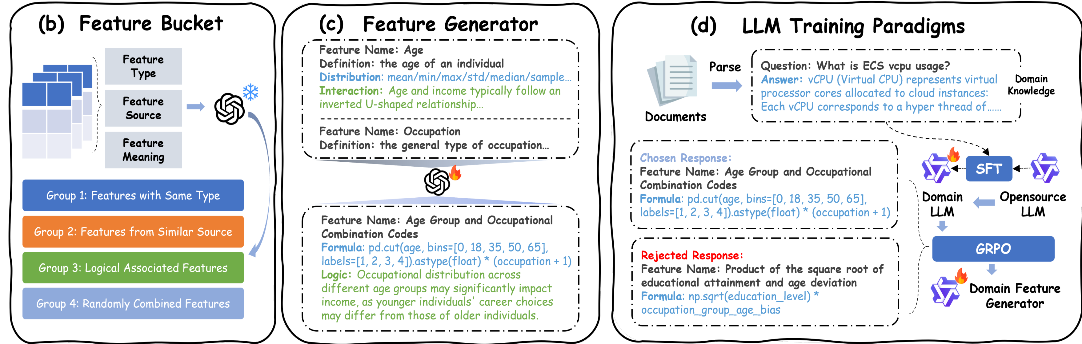
Domain-specific feature generation framework
