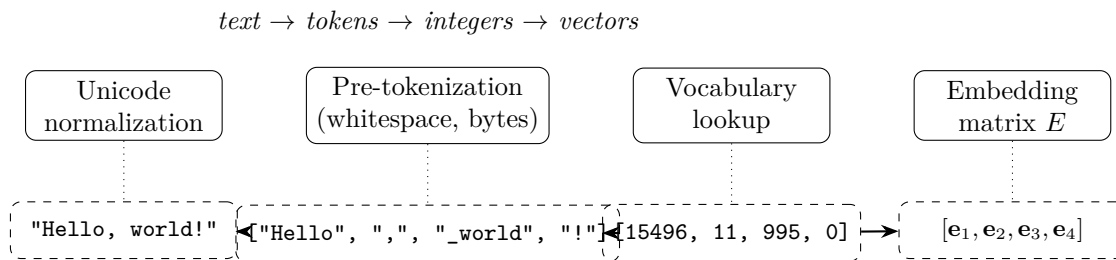
Figure 6: The tokenization pipeline: text is normalized, pre-tokenized, mapped to integer IDs via the vocabulary, and projected into \mathbb{R}^d through the embedding matrix E . After this step the model operates purely on dense vectors.
