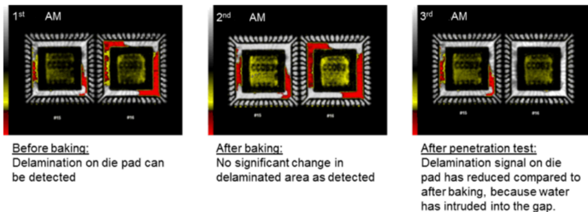
Figure D.1 — Acoustic microscopy (AM) scans of samples at different steps in the water penetration test
