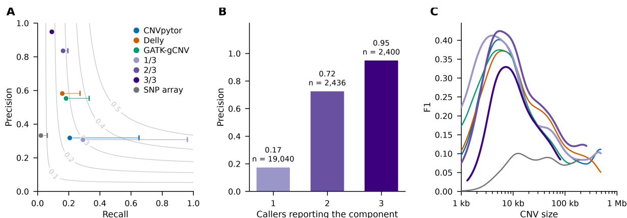
Figure 10: Performance of the 30x call sets and the SNP array against the merged benchmark at the adopted parameters. (A) Precision against recall, over grey F1 iso-contours. Each point sits on a bar running to its recall ceiling, the largest recall a call set of that size could attain. (B) Precision of the 1/3 consensus call set split by the number of callers that reported each component, taken over exactly that many callers rather than at least that many. (C) F1 against CNV size, smoothed in log-10 space over a bandwidth of 0.15 decades and drawn only where at least 50 calls contribute. Panels A and C share the legend in A.
