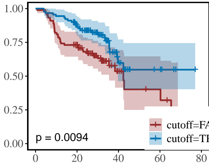
GEO_LUSC
