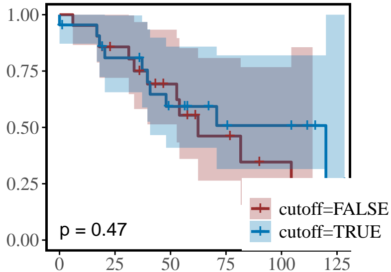
GEO_LUSC
