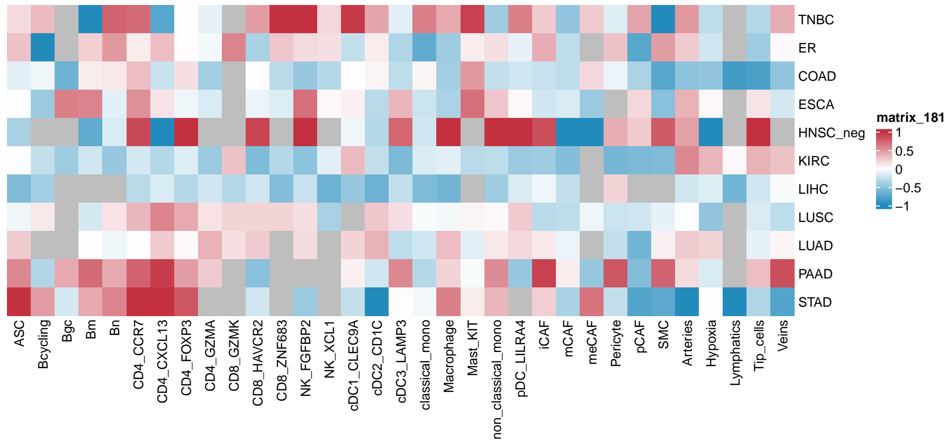
Heatmap of Gene Expression
