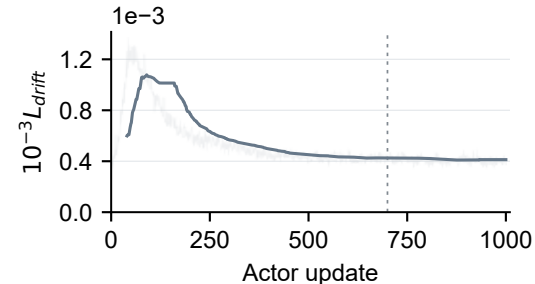
h Reconstructed drift
