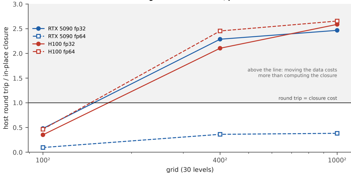
cost of reaching a host-side module, pinned PCIe 5.0
