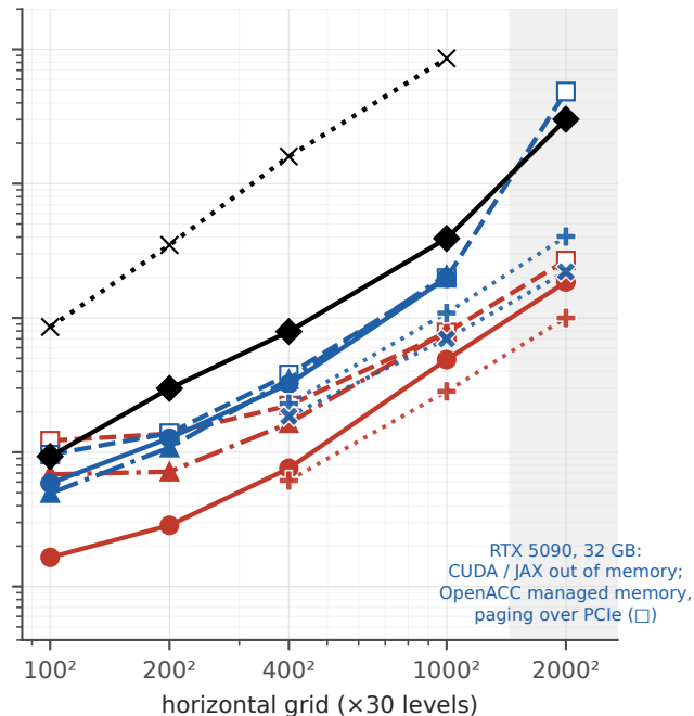
(b) with TKE closure + 3rd-order TVD (DC+TKE)
