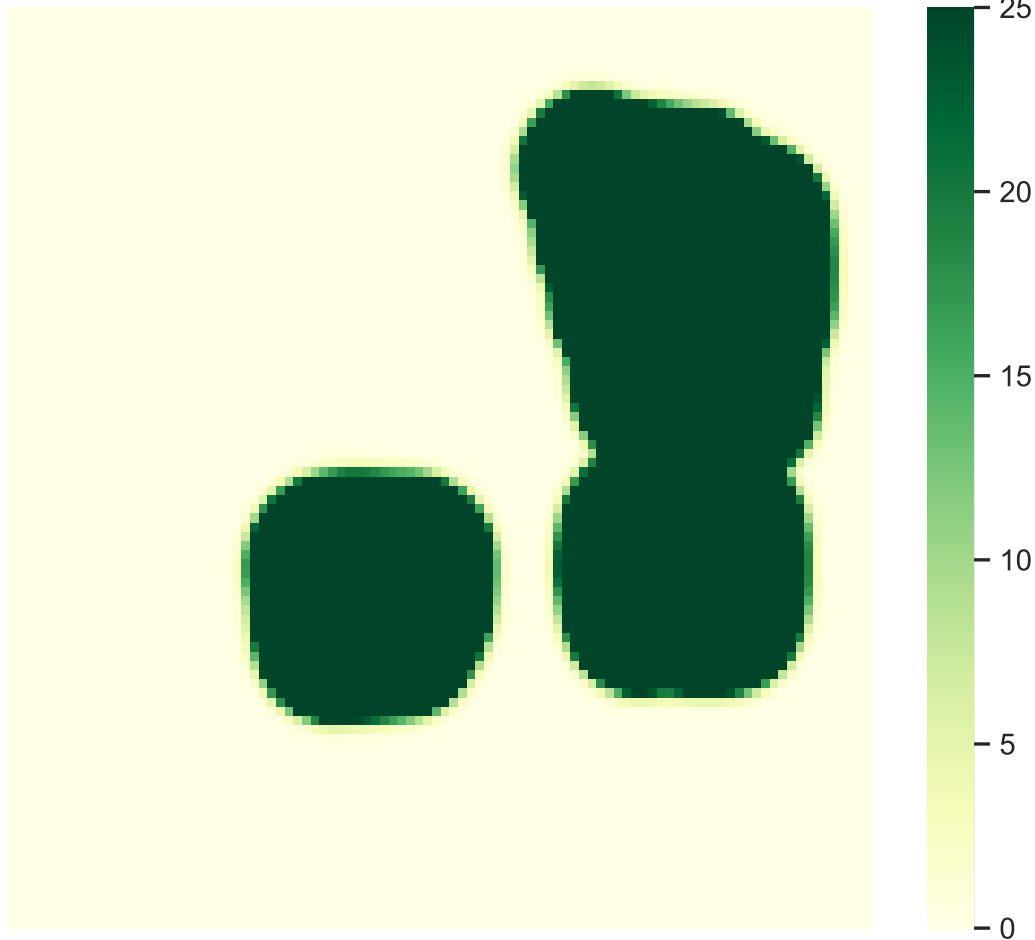
Mean population density (mean: 6.6)
