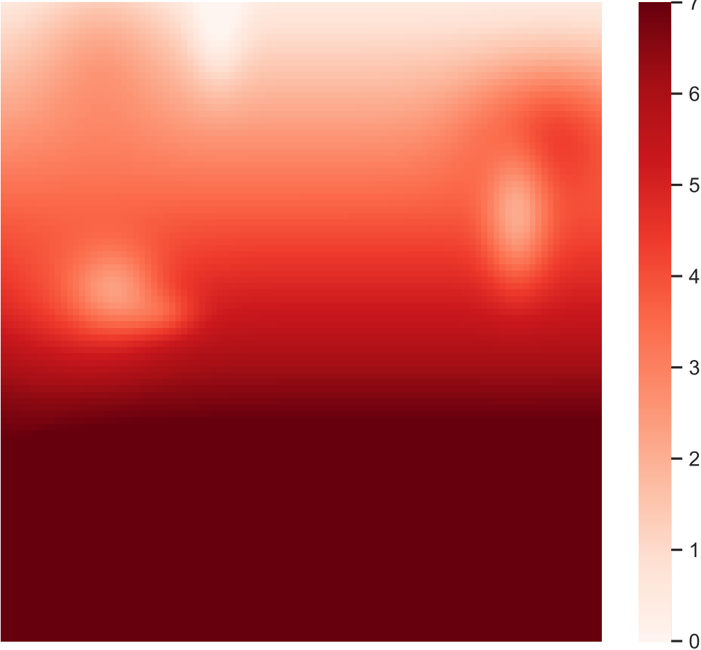
Mean annual temperature (mean anomaly: 5.39)
