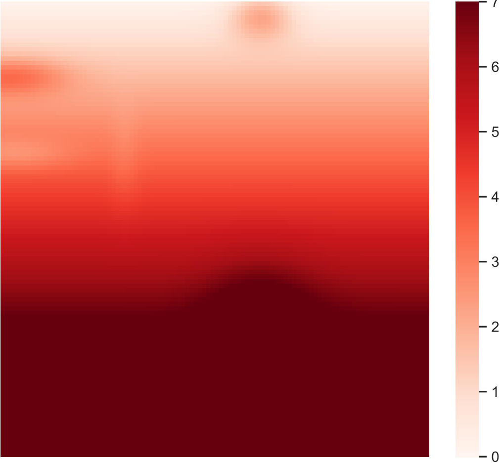
Mean annual temperature (mean anomaly: 5.17)
