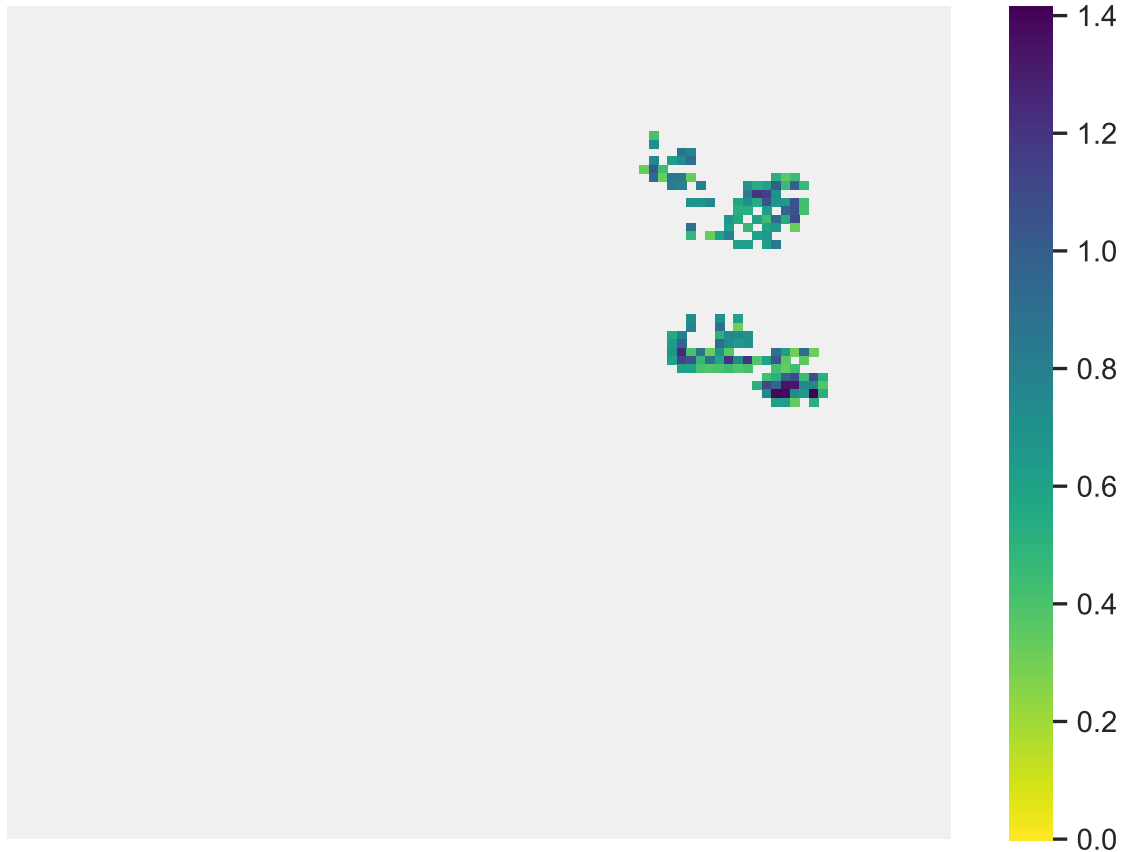
Sp. 5 (pop. size: 848, range size: 154)
