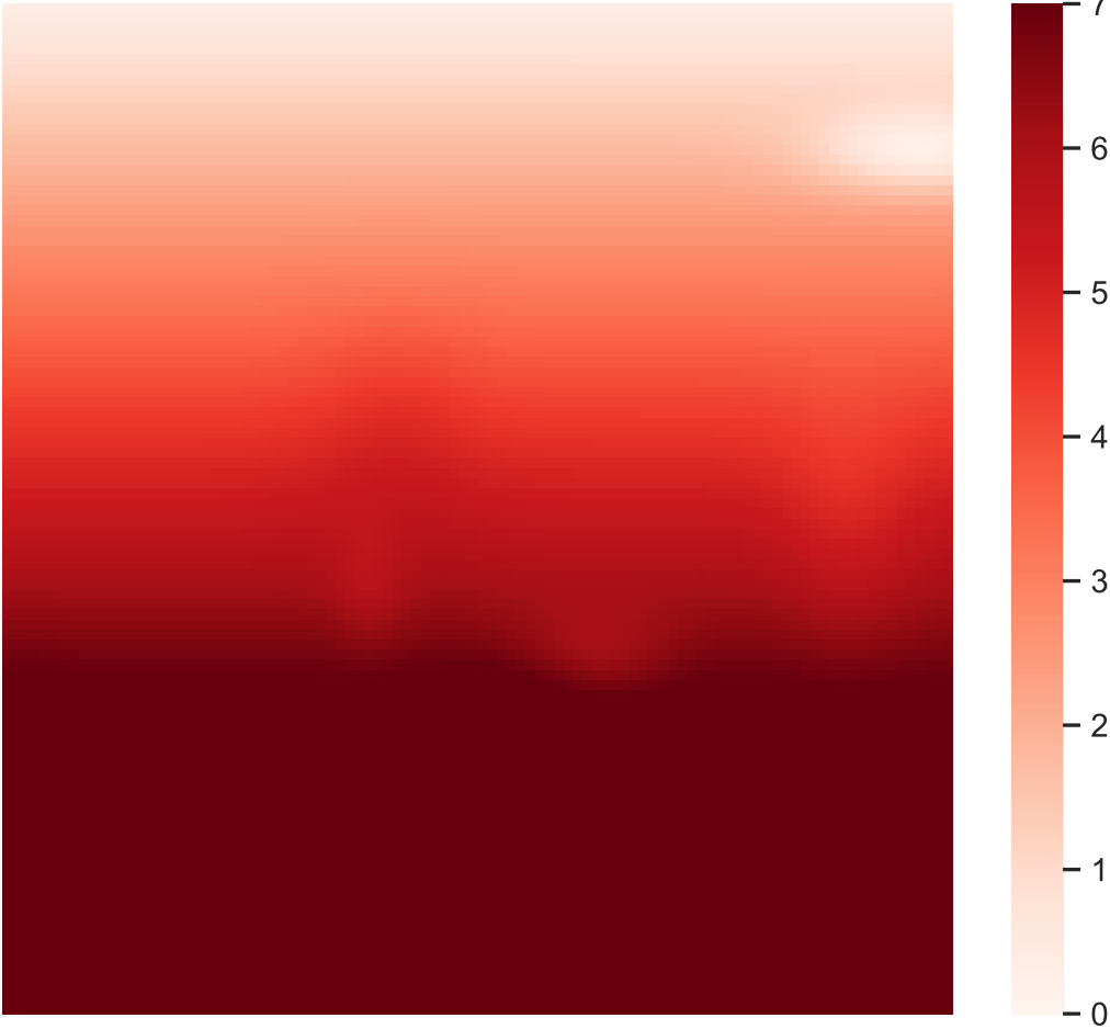
Mean annual temperature (mean anomaly: 5.27)
