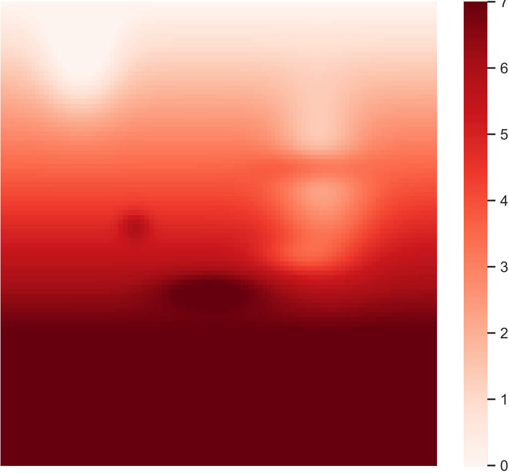
Mean annual temperature (mean anomaly: 4.83)
