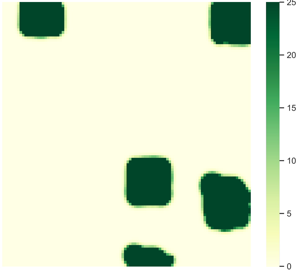
Mean population density (mean: 3.4)
