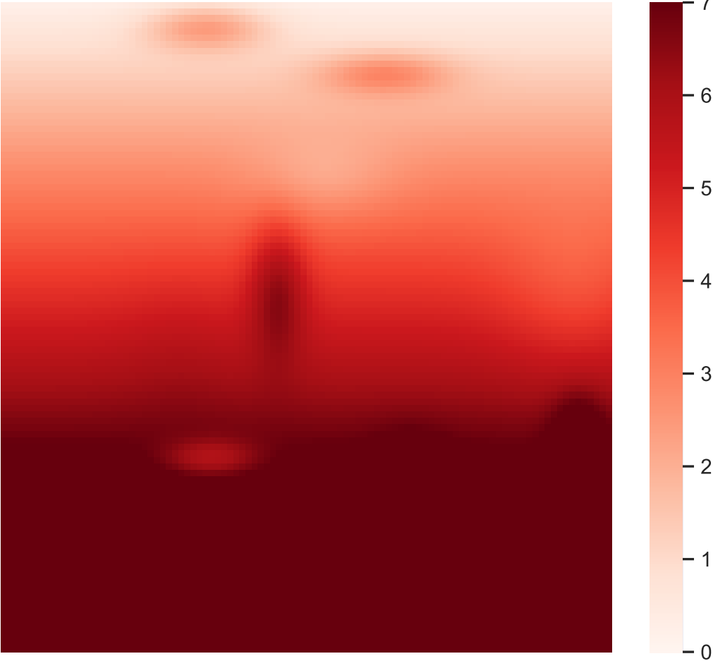
Mean annual temperature (mean anomaly: 5.25)
